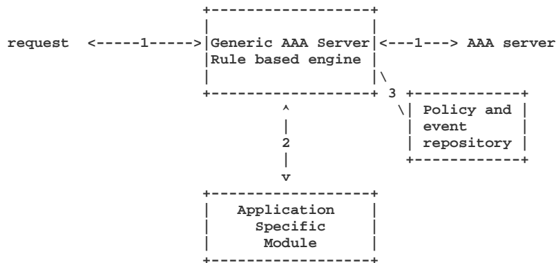
Fig. 2 -- Generic AAA Server Interactions
